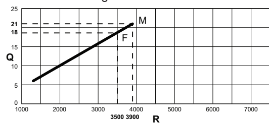
Afb.60 Belasting Avanta 24c
